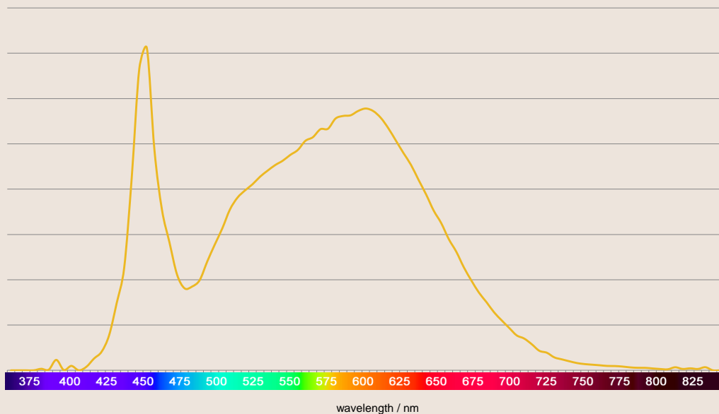
SPECTRAL POWER DISTRIBUTION OF LEDON 47W PANEL
